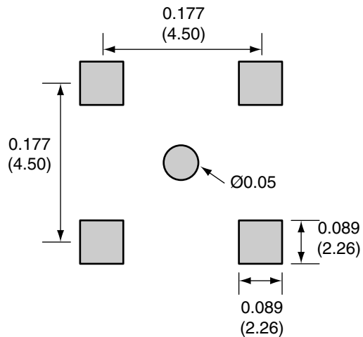
RECOMMENDED FOOTPRINT
